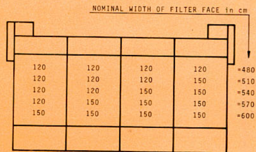
STANDARD ARRANGMENTS OF AUTOMATIC AIR FILTERS. OTHER VARIATIONS AVAILABLE.
