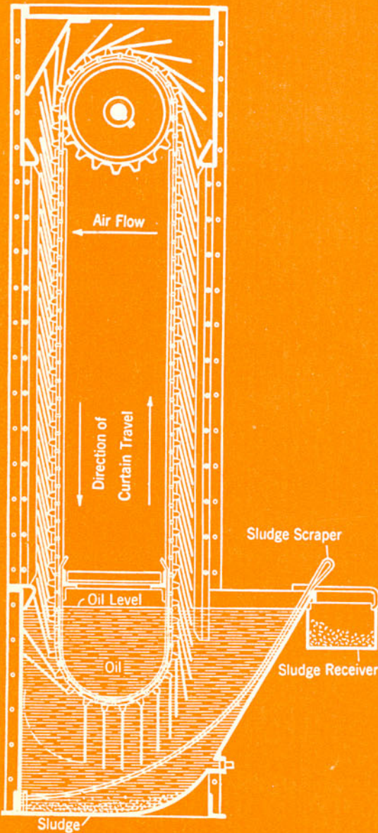
CONTINUOUS BELT FILTER
